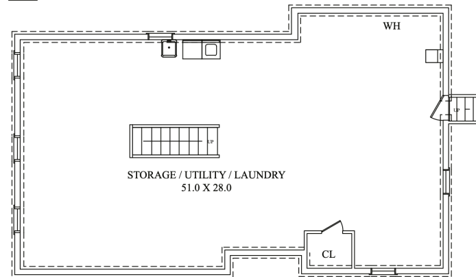
LOWER LEVEL
