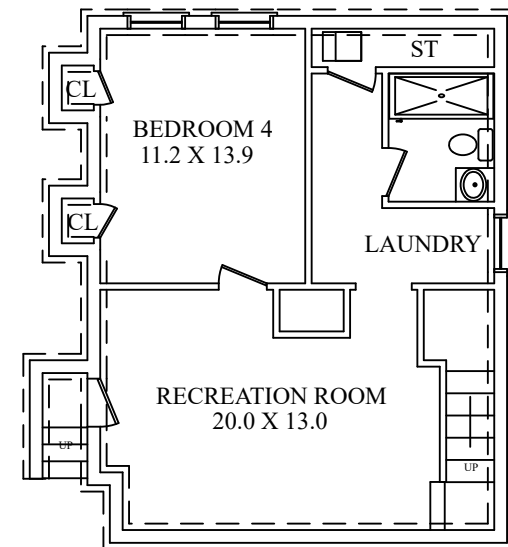
LOWER LEVEL
