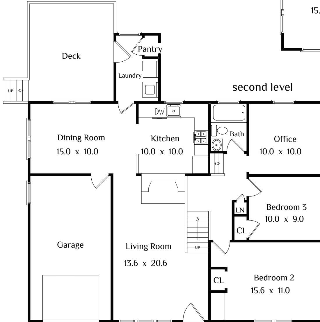
FIRST LEVEL
