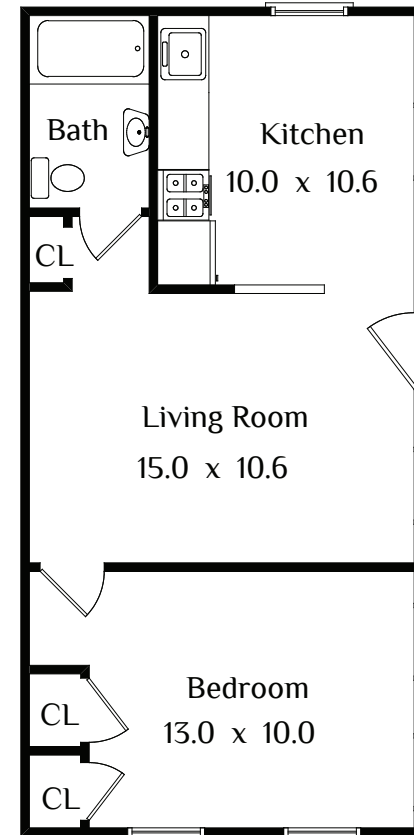
APARTMENT
